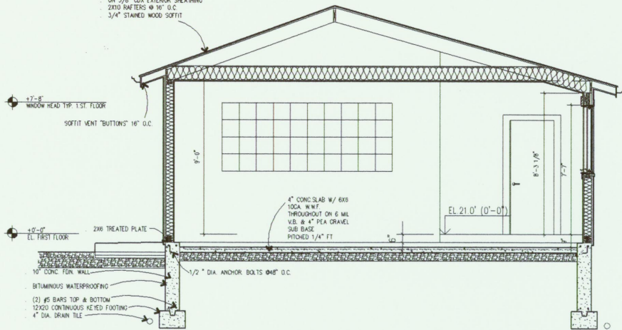
1 NORTH-EAST/SOUTH-WEST SECTION @ GARAGE SCALE : 3/8" = 1'-0"
